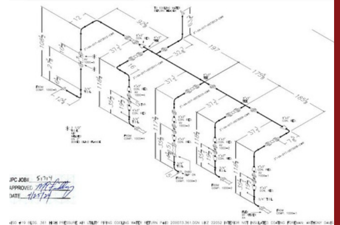
CAD Isometrics for design-build & layout services
