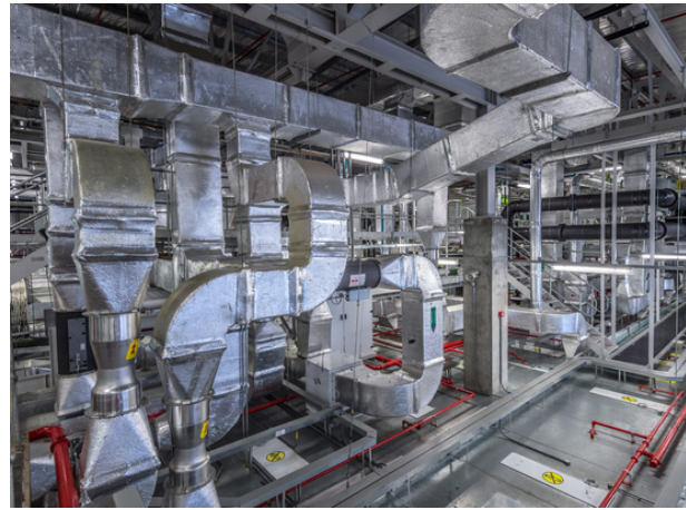
SMANCA Standard Duct Work Installed and Insulated
