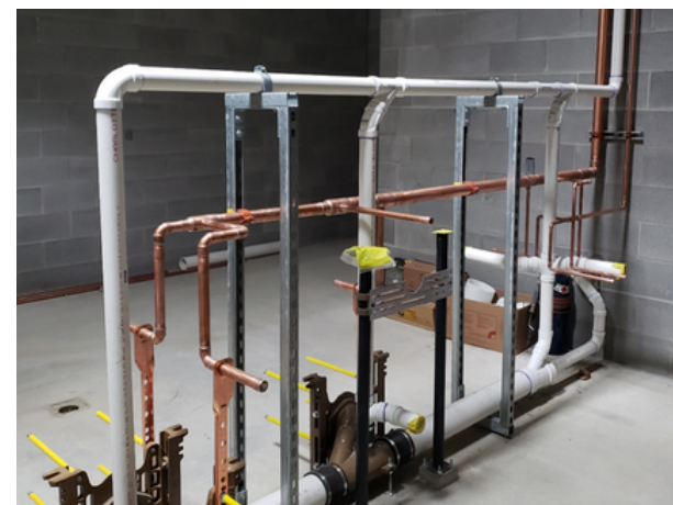
Back-to-back bathroom rough-in
